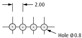
Recommended PC Board Pattern
